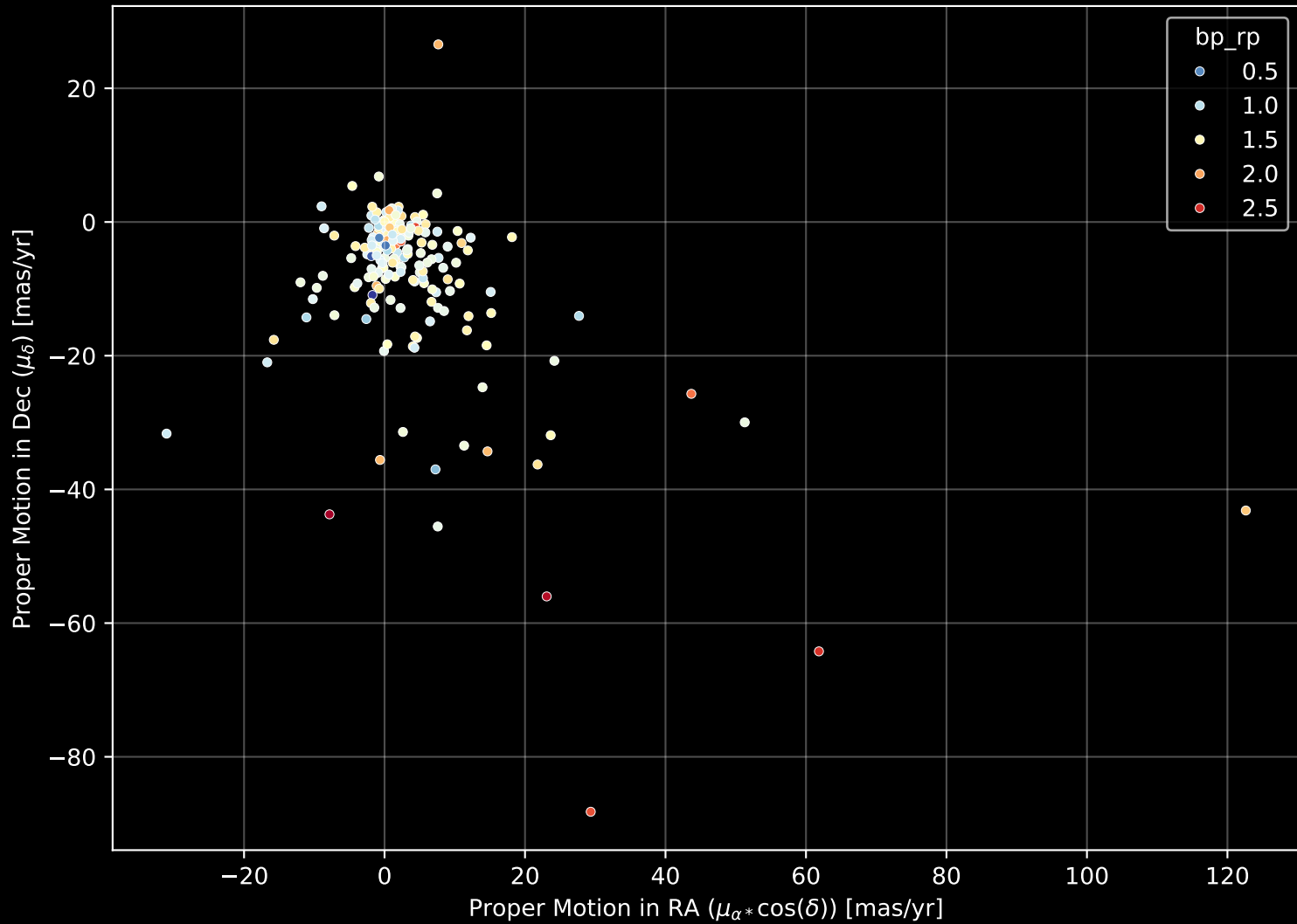
APOGEE DR17 Field: [K2_C13_180-12_bt] Proper Motion Diagram (n= 208)
