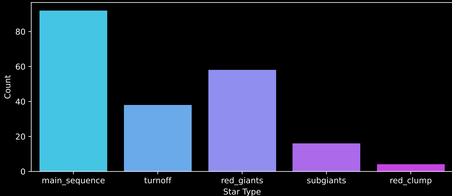
APOGEE DR17 Field: [K2_C13_180-12_btx] Count plot of Star Type
