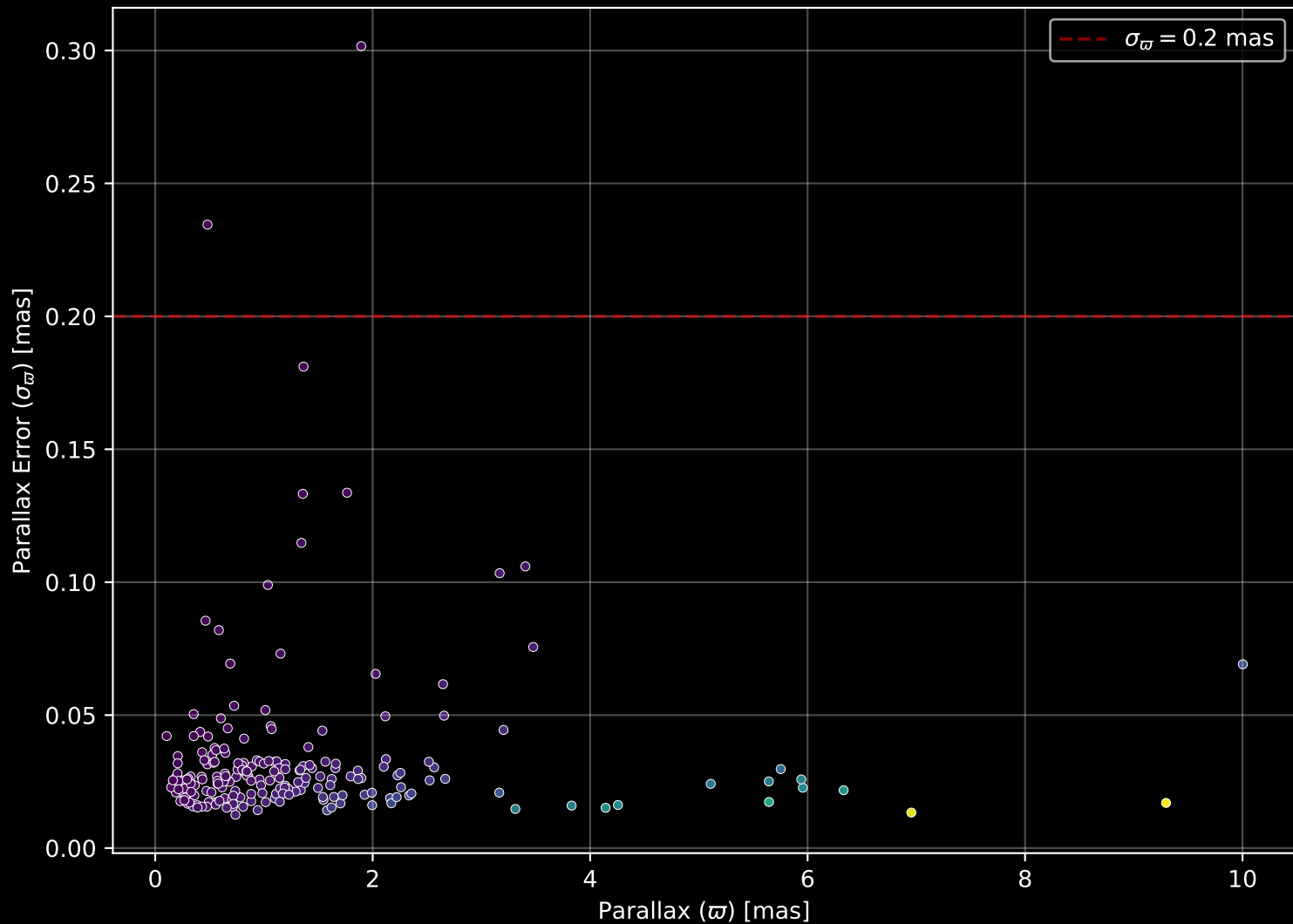
APOGEE DR17 Field: [K2_C13_180-12_btx] Parallax Quality (n= 208)
