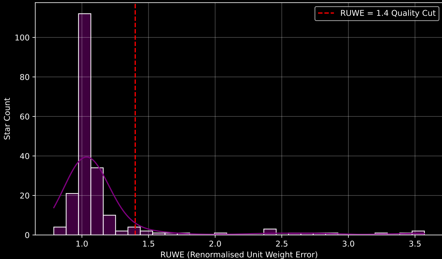
GAPOGEE DR17 Field [K2_C13_180-12_btx] RUWE Distribution (n= 204)
