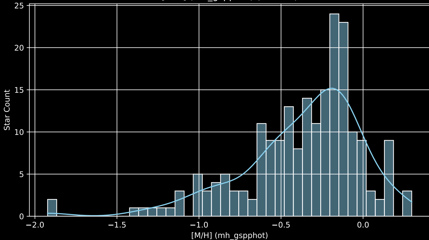
APOGEE DR17 Field: [K2_C13_180-12_btx [M/H] (mh_gspphot) (n= 208)
