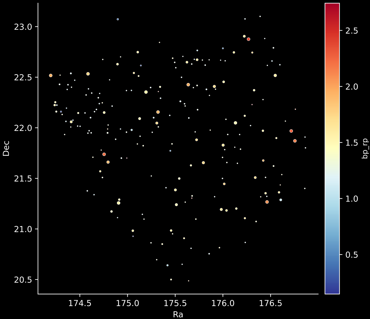
APOGEE DR17 Field: [K2_C13_180-12_btx] Stars: 208
